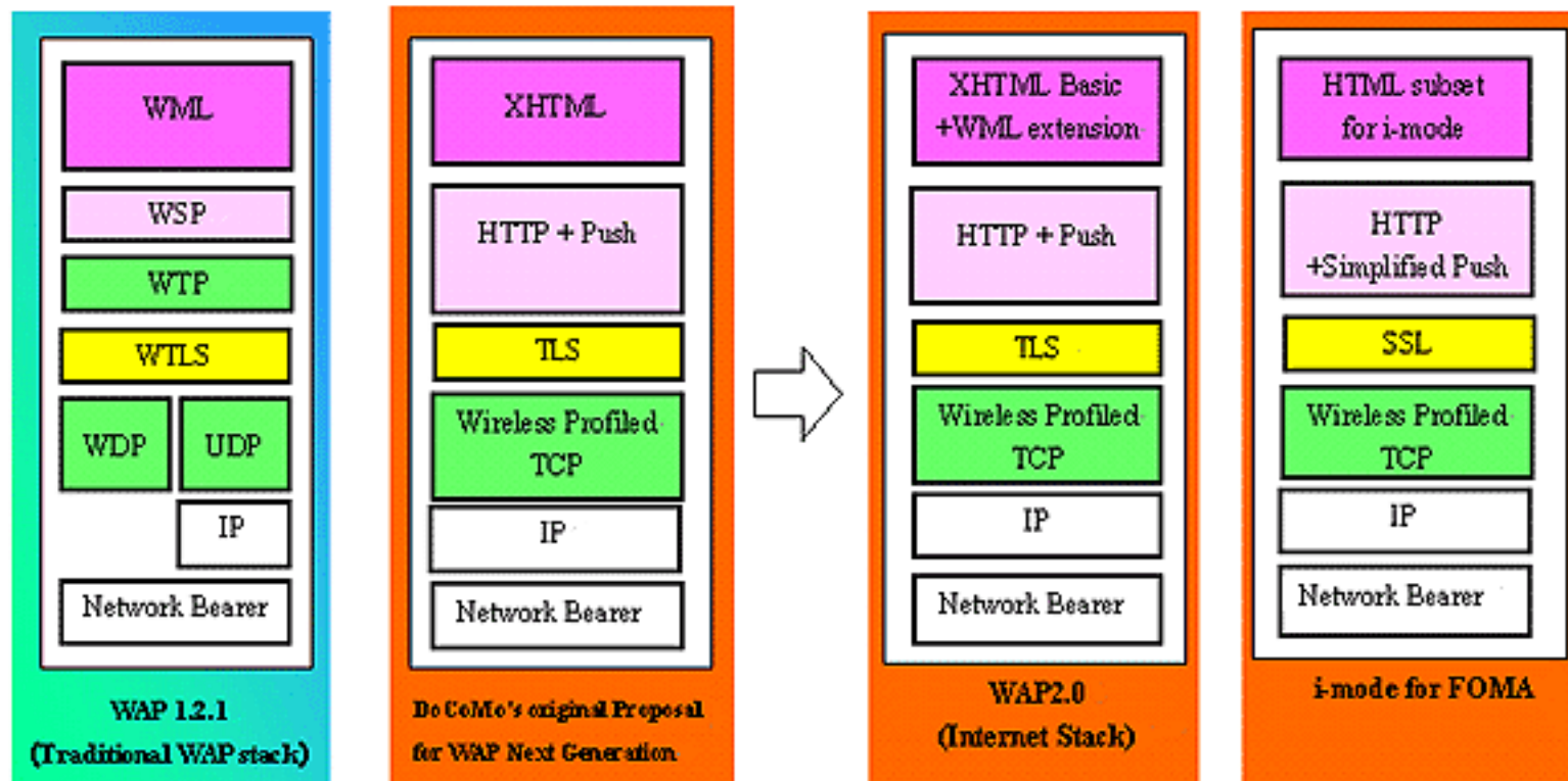
Protocol Stack for WAP2.0 in comparison with WAP1.2.1 and i-mode for FOMA
